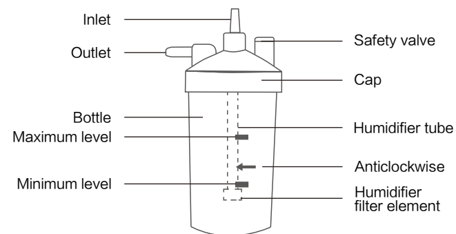
Figure 5: Humidifier Components
